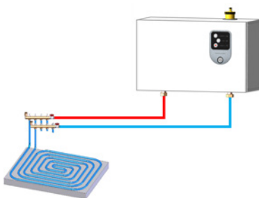
PLANCHER CHAUFFANT
